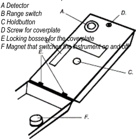
The controls and other parts of the Photometer
